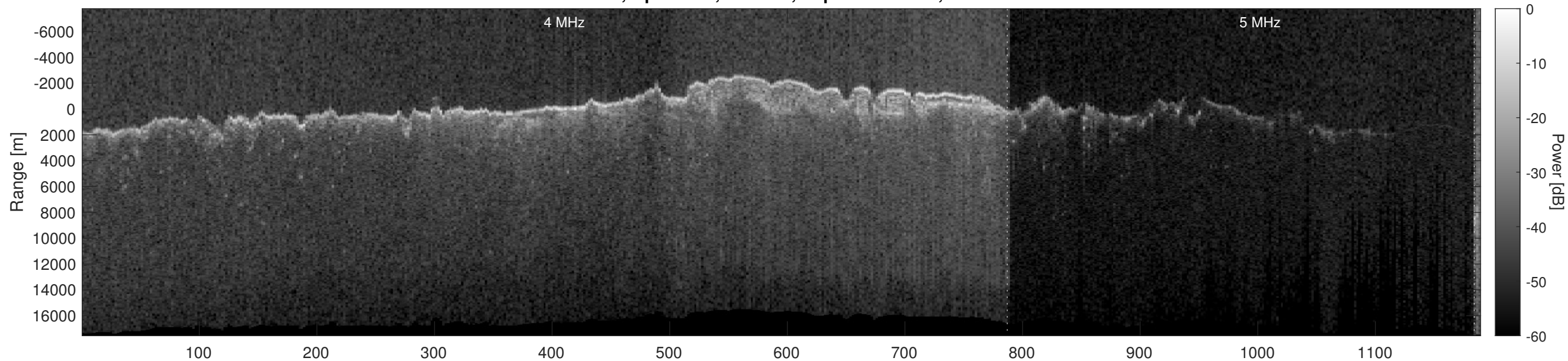
Orbit 10829, Optimized, Window, Depth-Corrected, Channel 2
