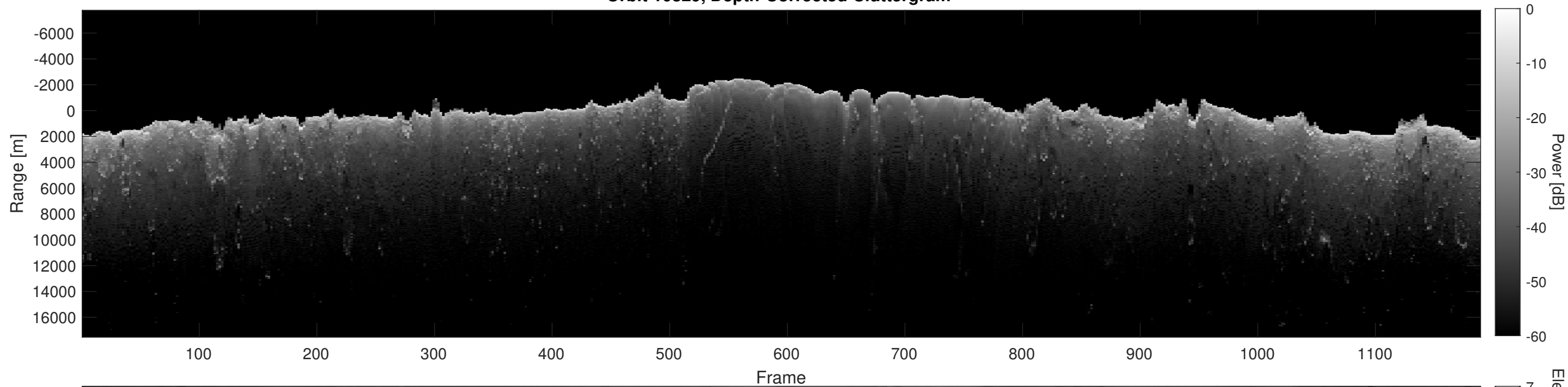
Orbit 10829, Depth-Corrected Cluttergram
