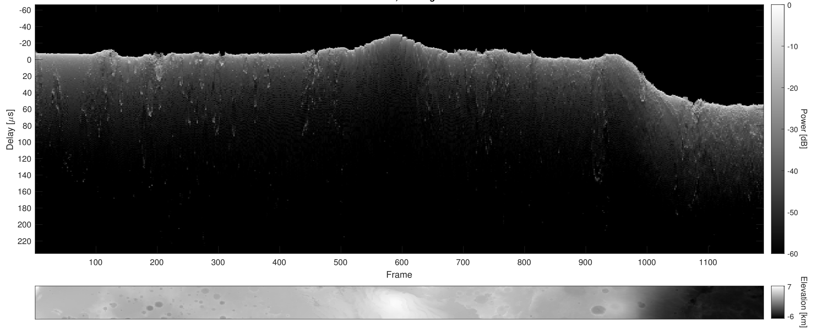
Orbit 10830, Cluttergram
