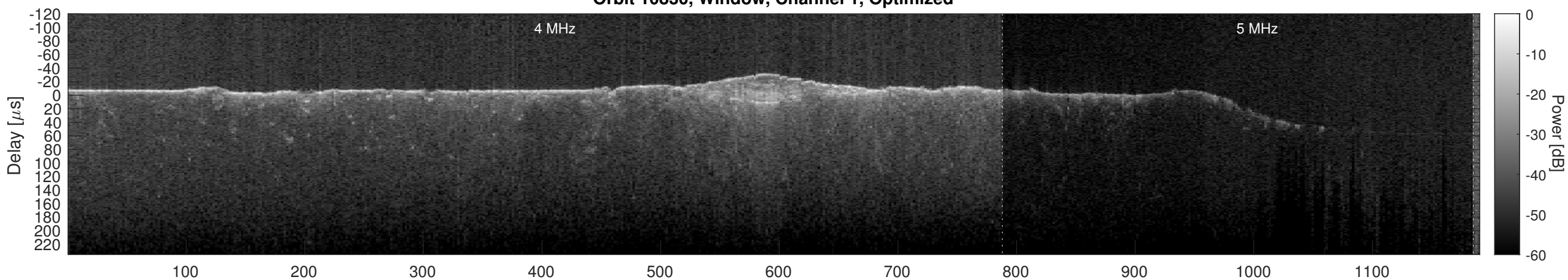
Orbit 10830, Cluttergram
