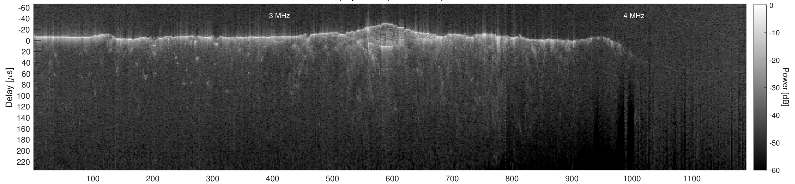
Orbit 10830, Cluttergram
