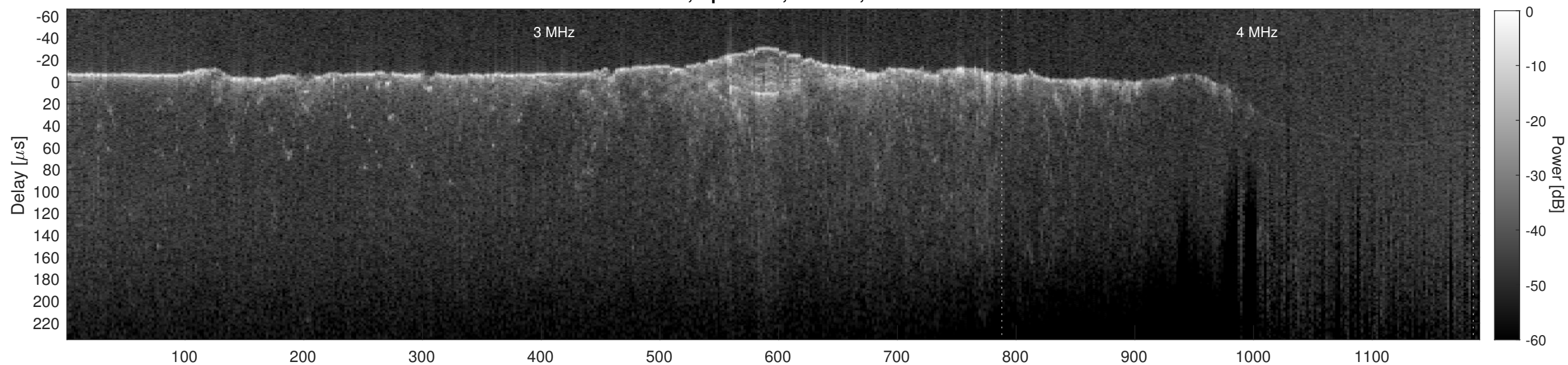
Orbit 10830, Cluttergram
