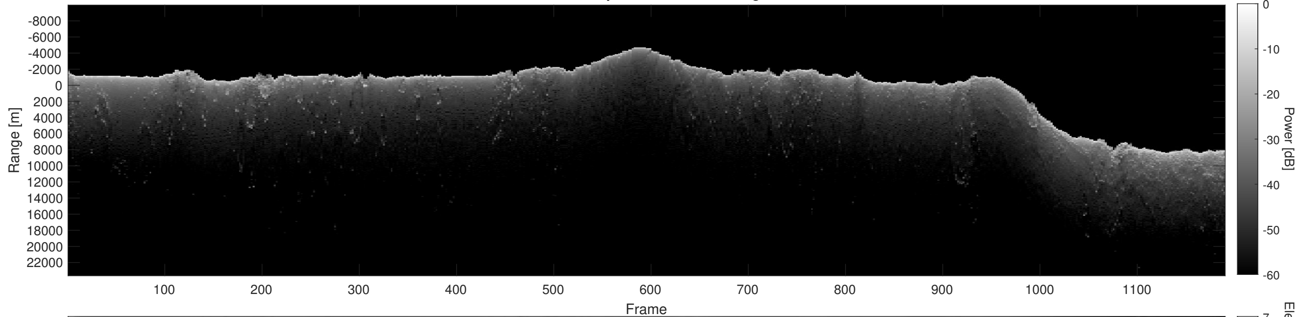
Orbit 10830, Depth-Corrected Cluttergram
