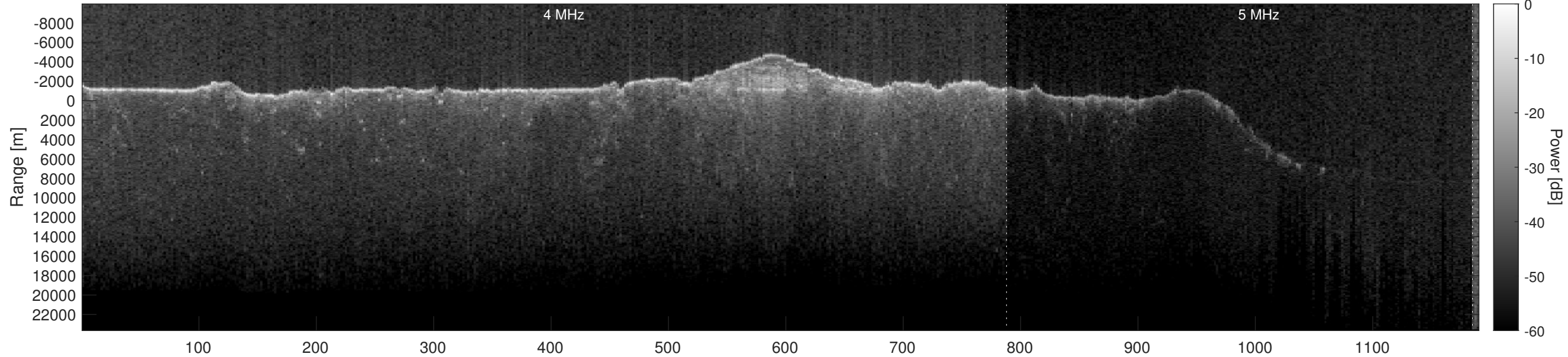
Orbit 10830, Optimized, Window, Depth-Corrected, Channel 2
