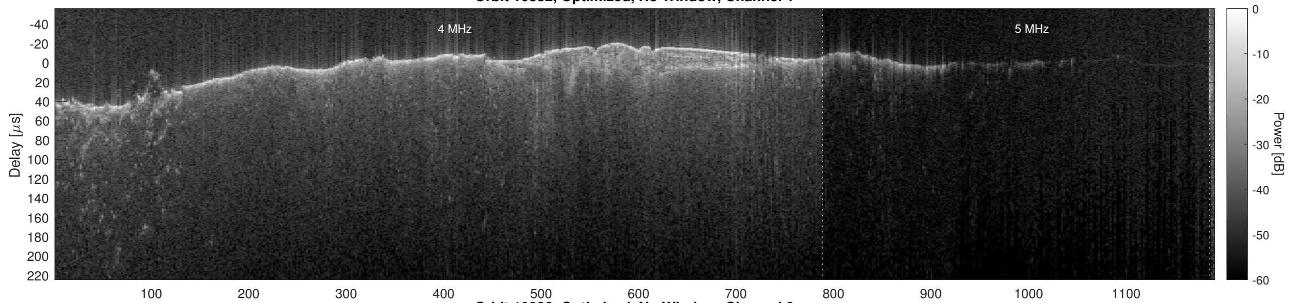
Orbit 10832, Optimized, No Window, Channel 2
