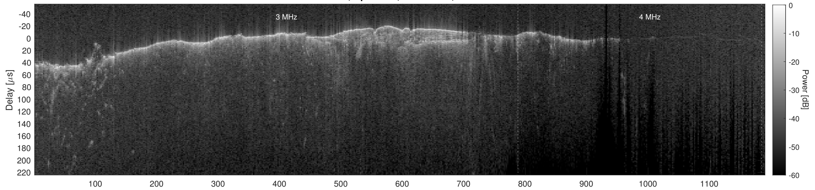
Orbit 10832, Cluttergram
