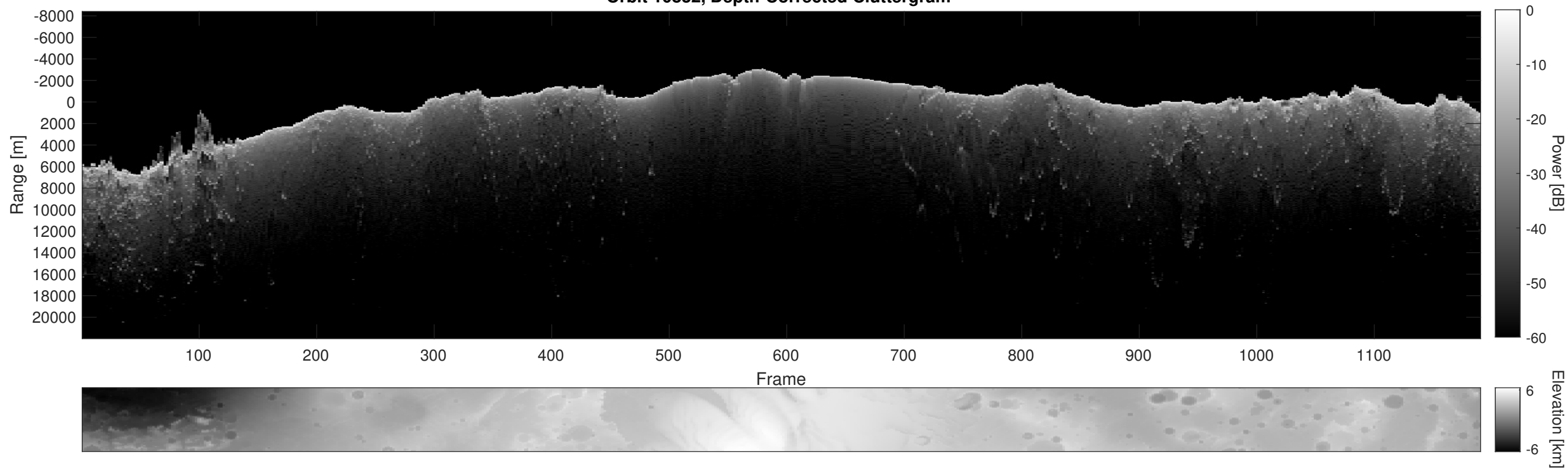
Orbit 10832, Depth-Corrected Cluttergram
