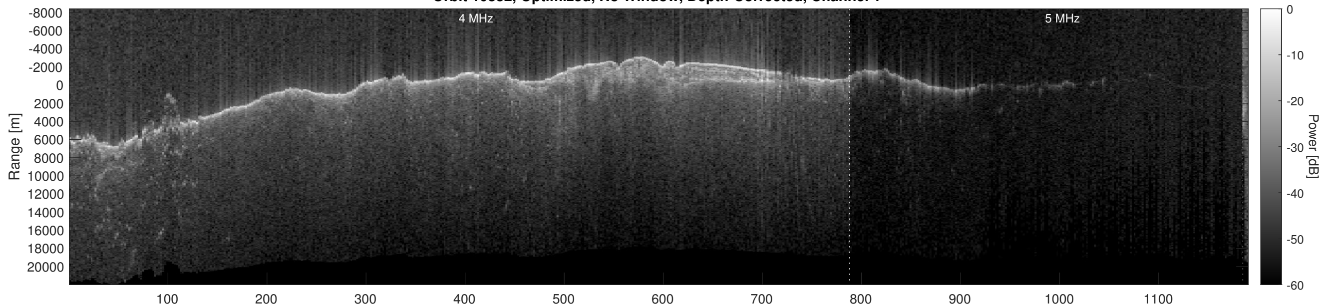
Orbit 10832, Optimized, No Window, Depth-Corrected, Channel 2
