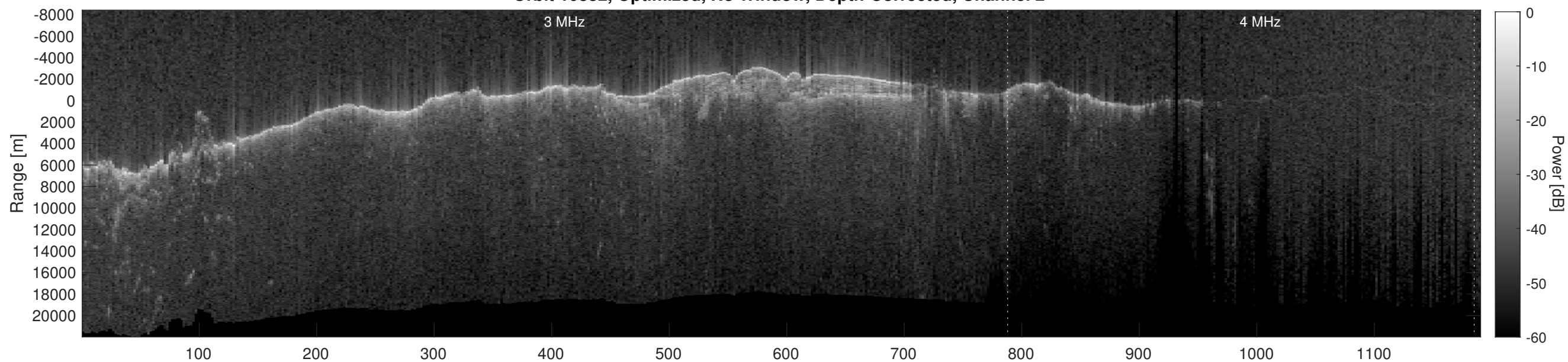
Orbit 10832, Depth-Corrected Cluttergram
