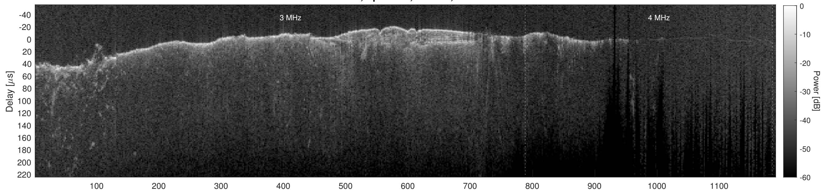
Orbit 10832, Cluttergram
