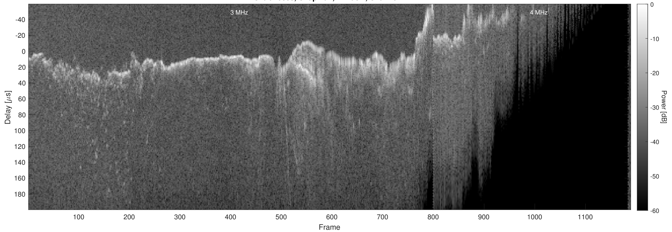
Orbit 10833, Chapman, Window, Channel 2
