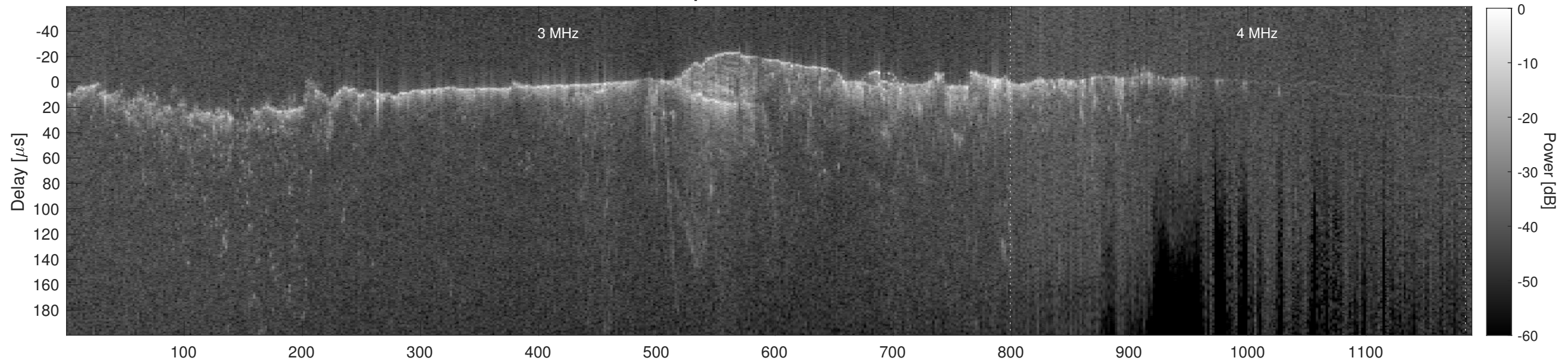
Orbit 10833, Cluttergram
