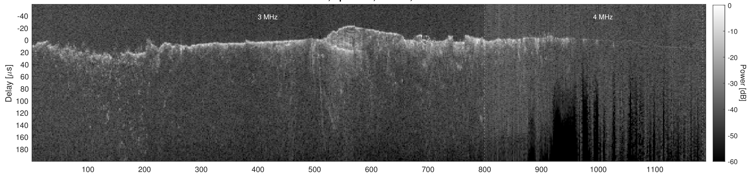
Orbit 10833, Cluttergram
