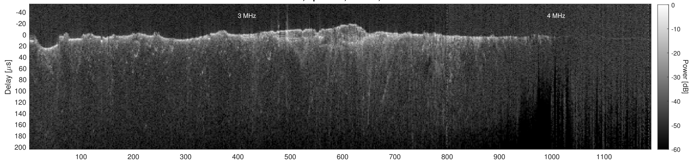
Orbit 10834, Cluttergram
