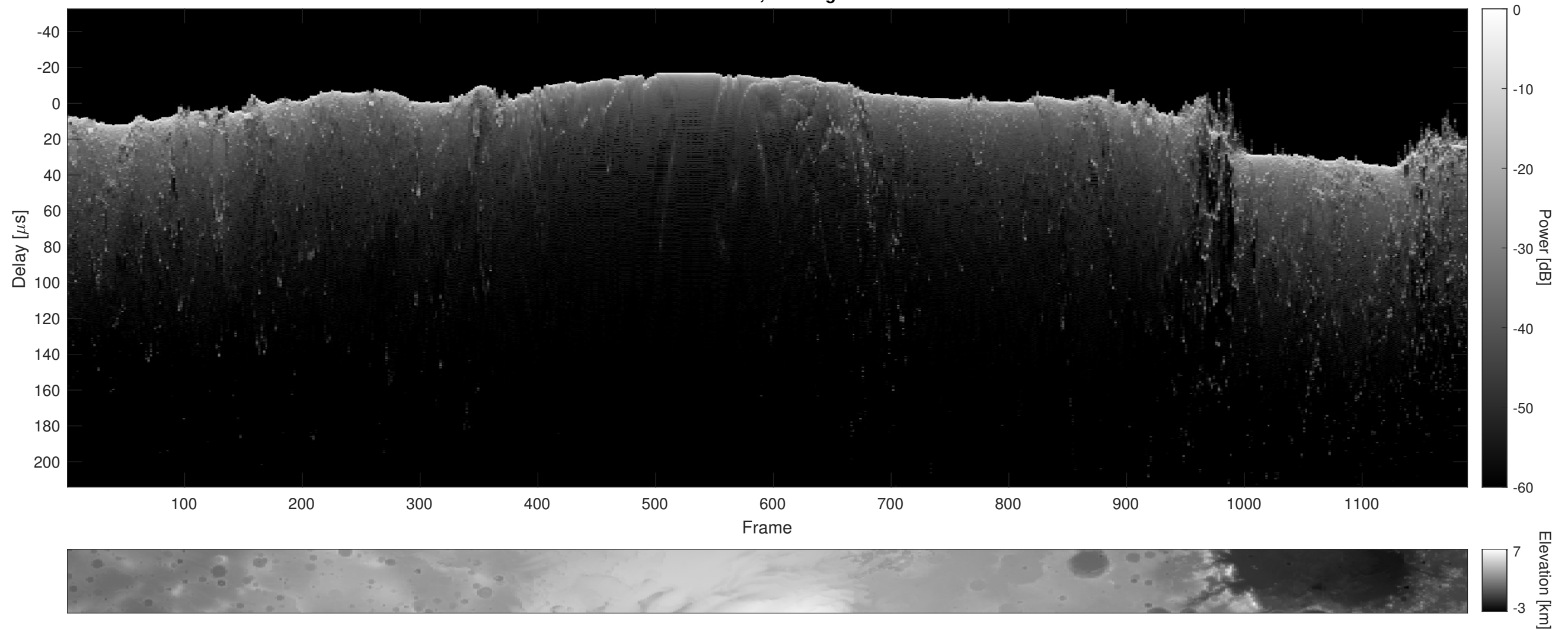
Orbit 10838, Cluttergram
