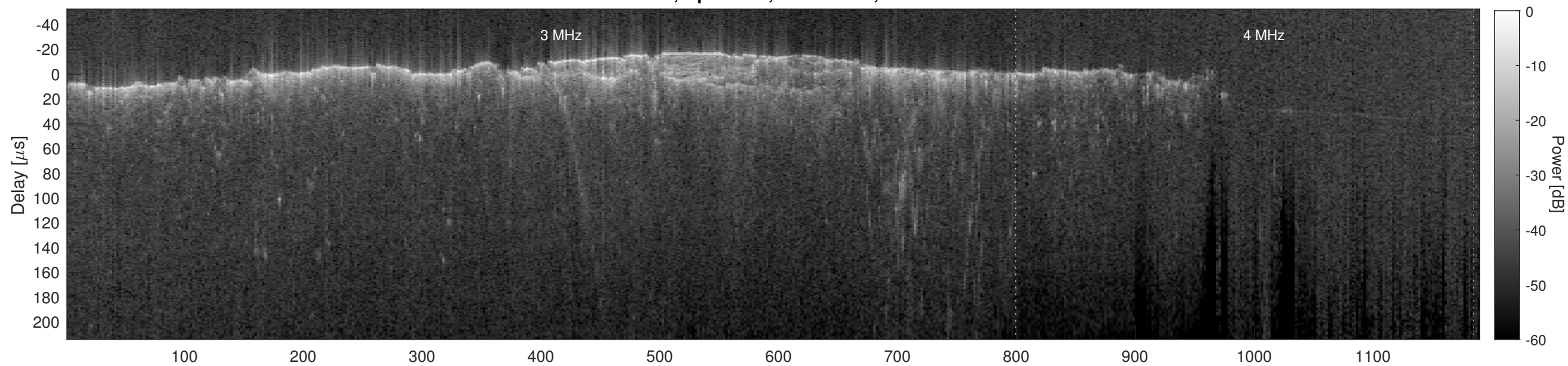
Orbit 10838, Cluttergram
