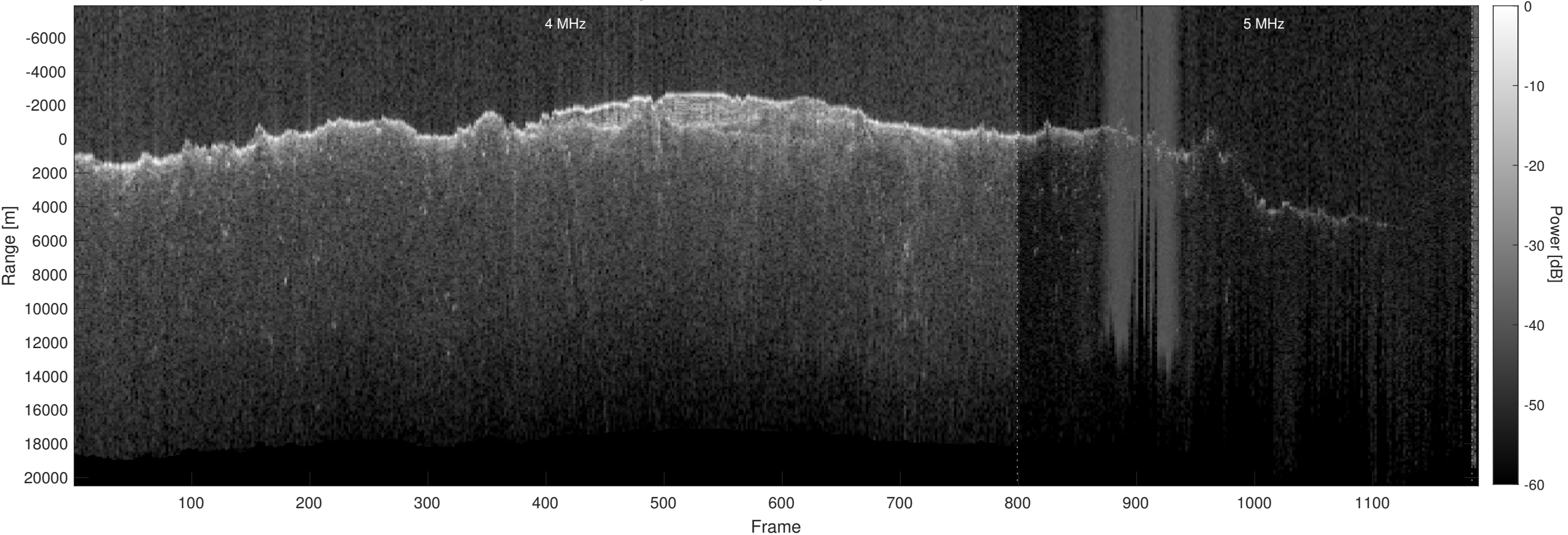
Orbit 10838, Optimized, Window, Depth-Corrected, Channel 2
