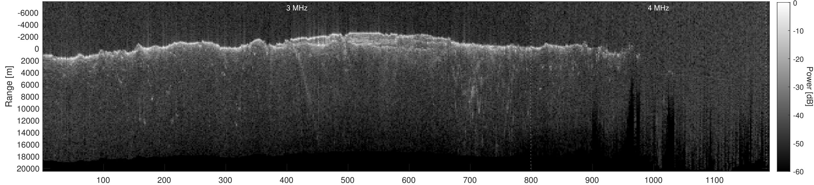
Orbit 10838, Depth-Corrected Cluttergram
