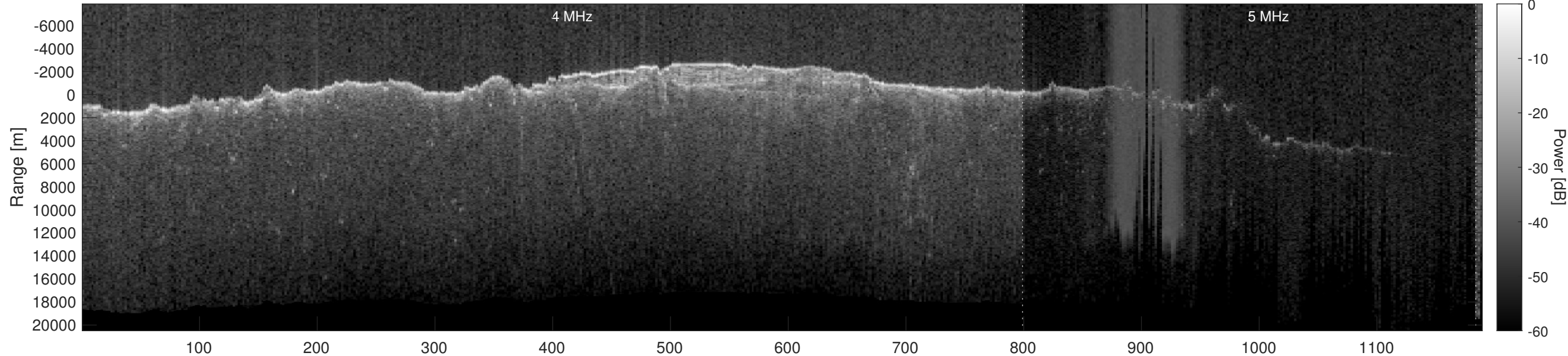
Orbit 10838, Optimized, Window, Depth-Corrected, Channel 2
