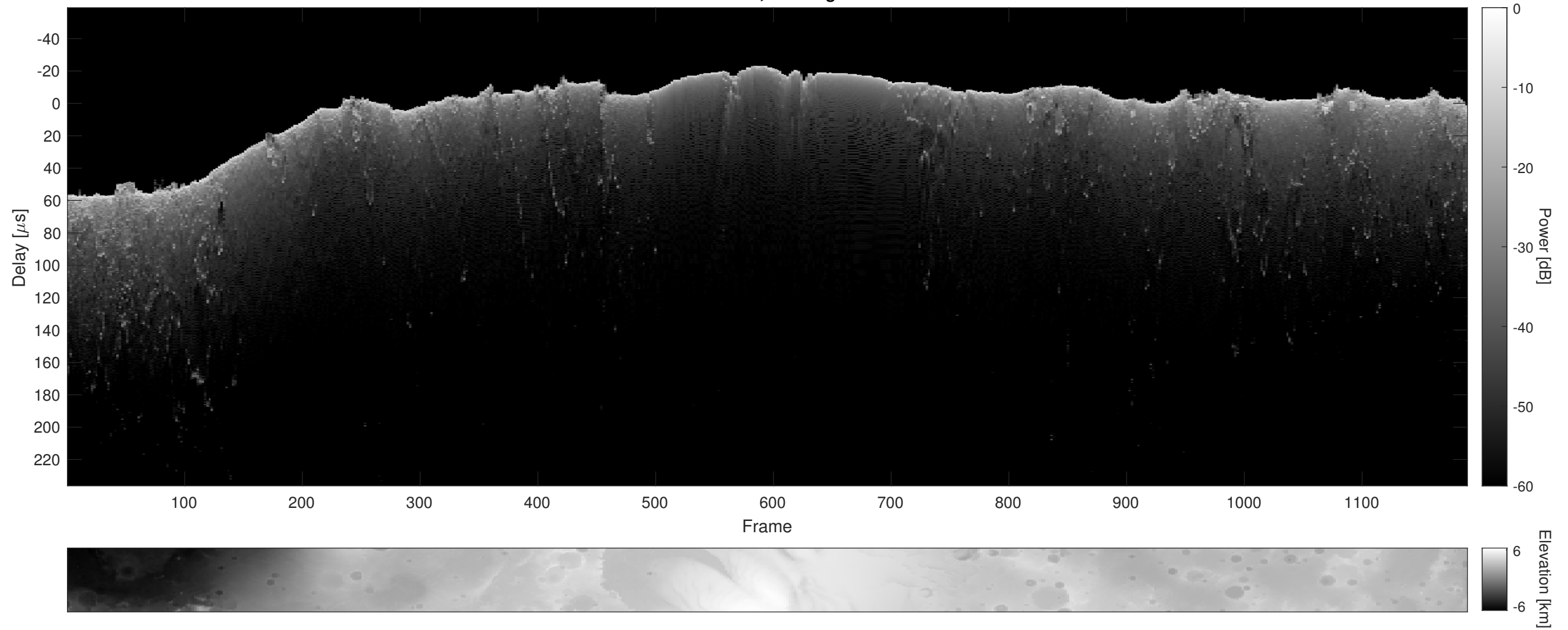
Orbit 10839, Cluttergram
