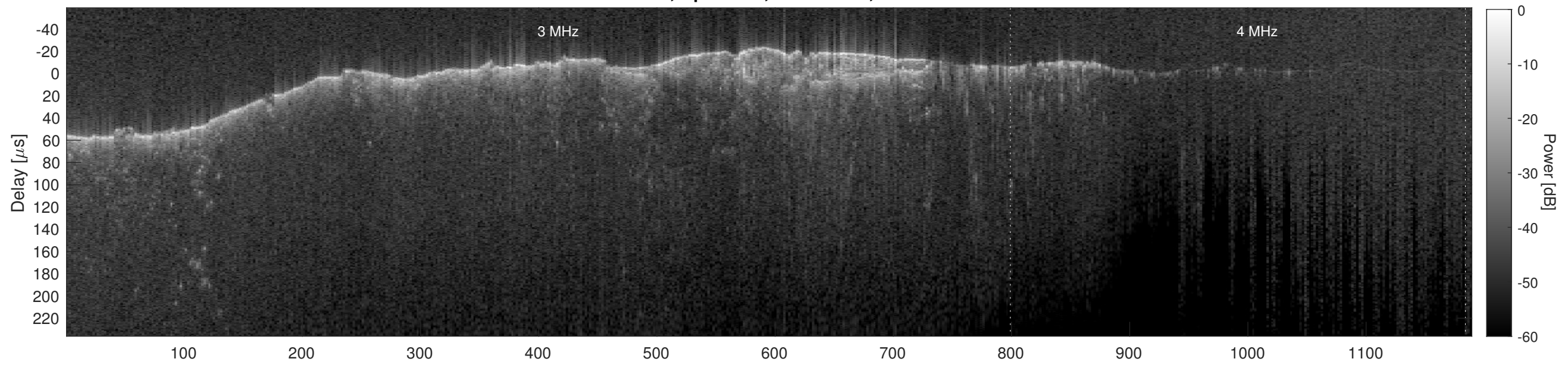
Orbit 10839, Cluttergram
