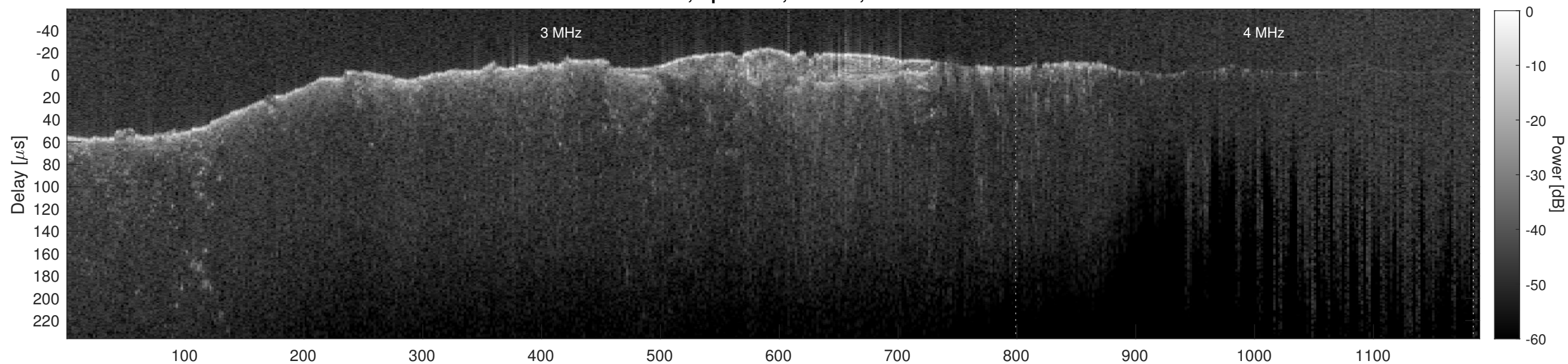
Orbit 10839, Cluttergram
