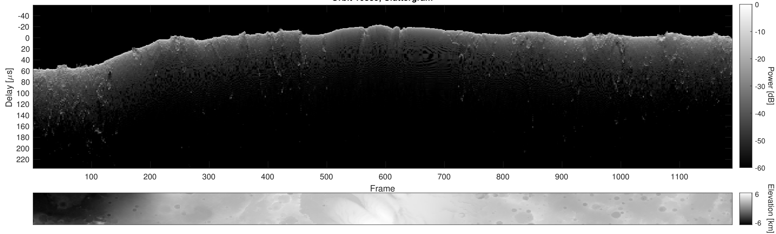
Orbit 10839, Cluttergram
