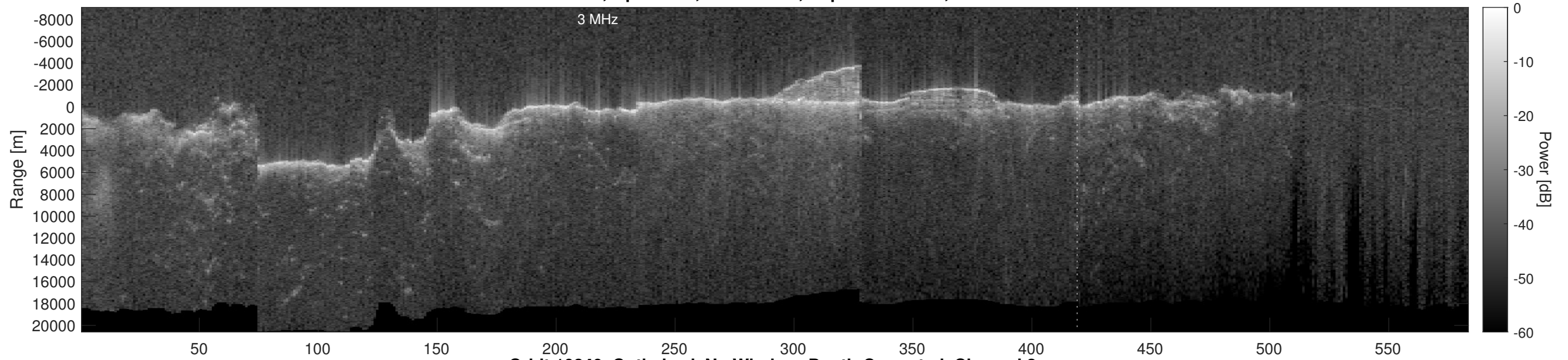
Orbit 10840, Optimized, No Window, Depth-Corrected, Channel 2
