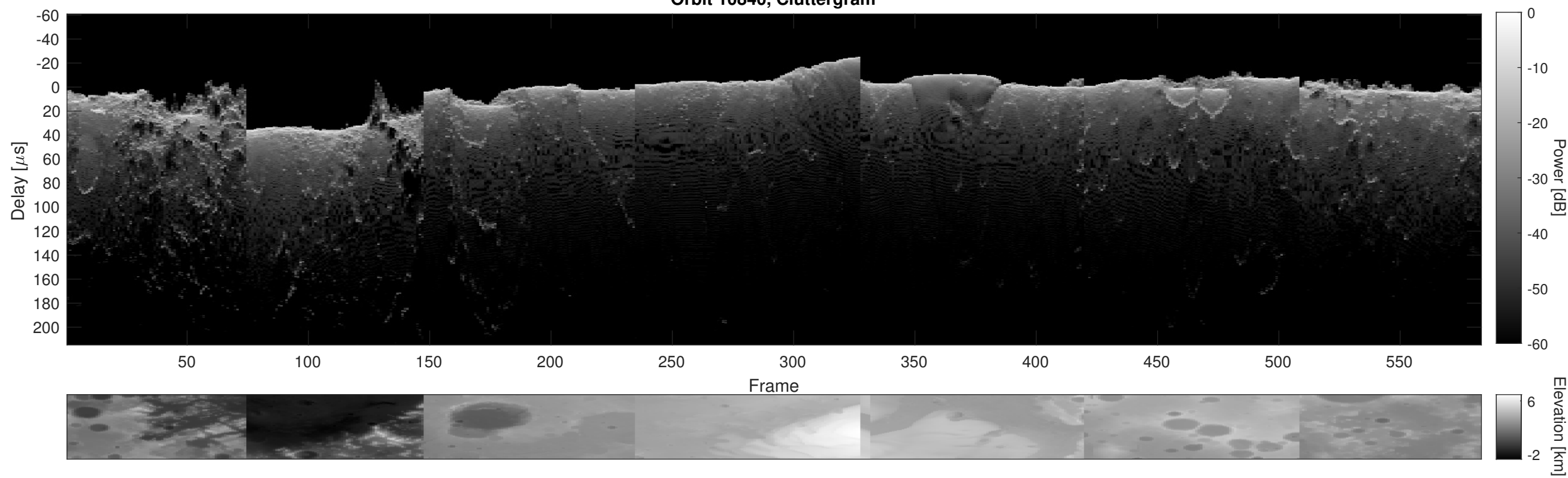
Orbit 10840, Cluttergram
