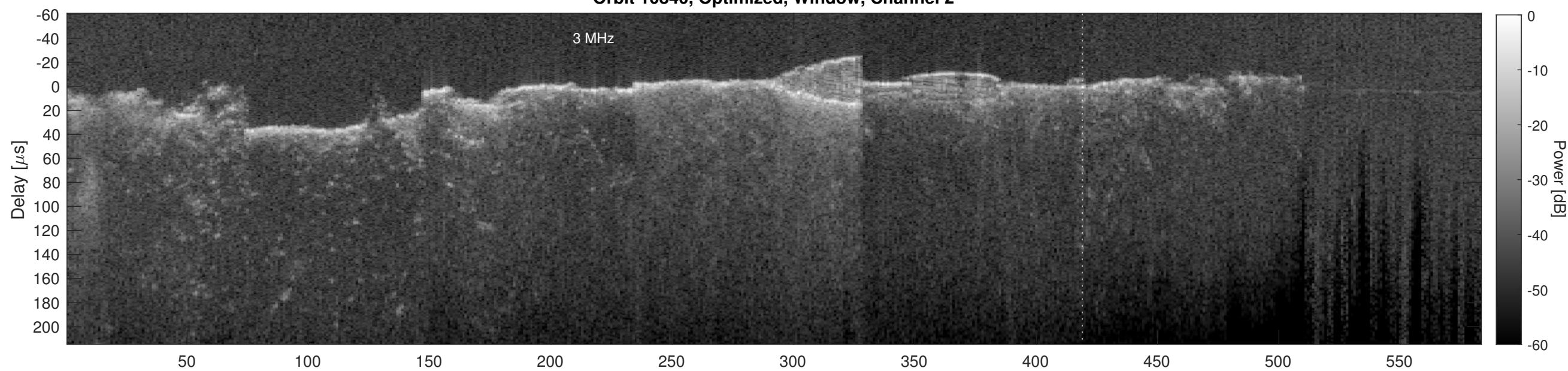
Orbit 10840, Cluttergram
