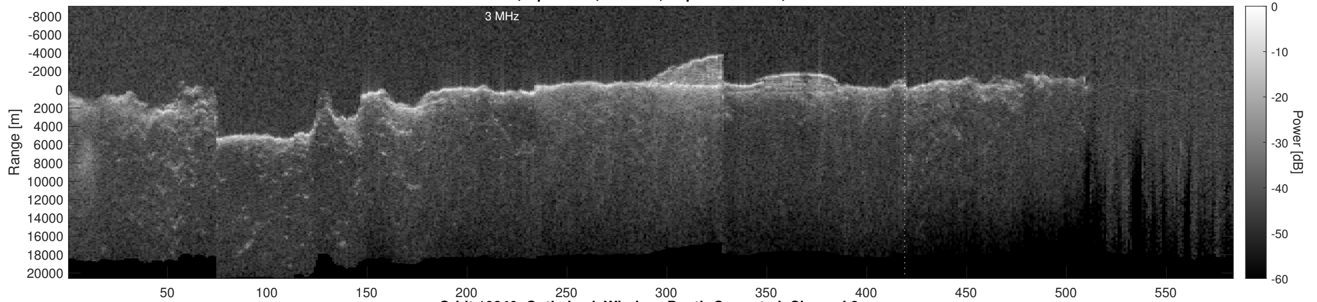
Orbit 10840, Optimized, Window, Depth-Corrected, Channel 2
