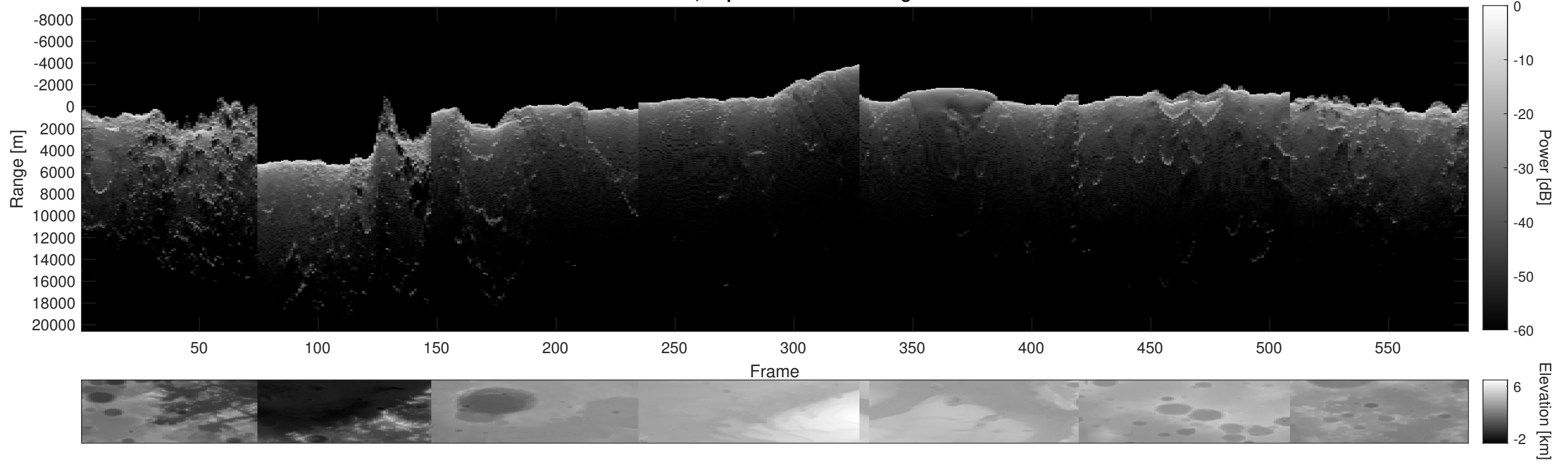
Orbit 10840, Depth-Corrected Cluttergram
