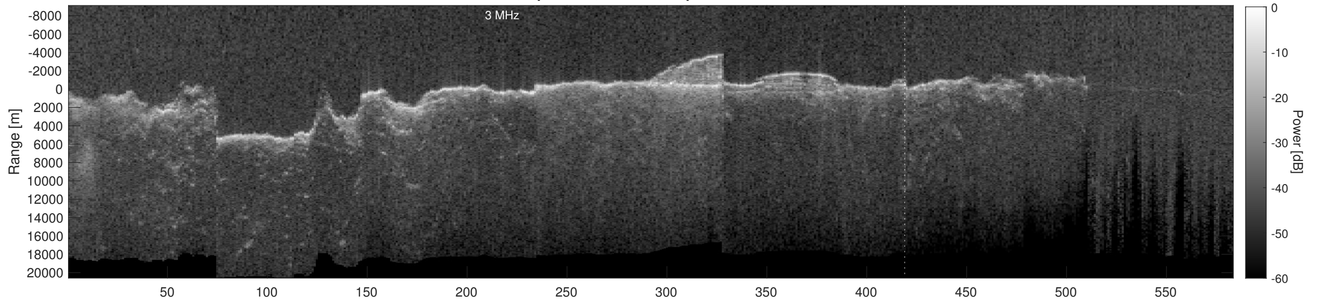
Orbit 10840, Depth-Corrected Cluttergram
