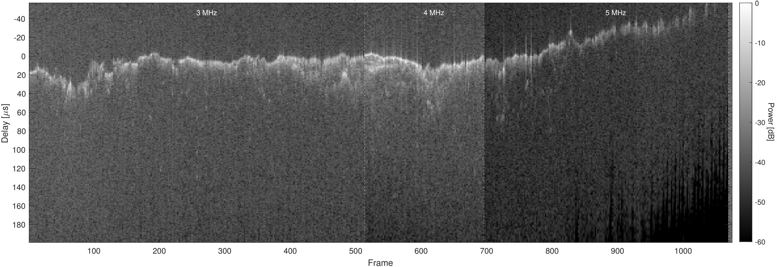
Orbit 10842, Chapman, No Window, Channel 2
