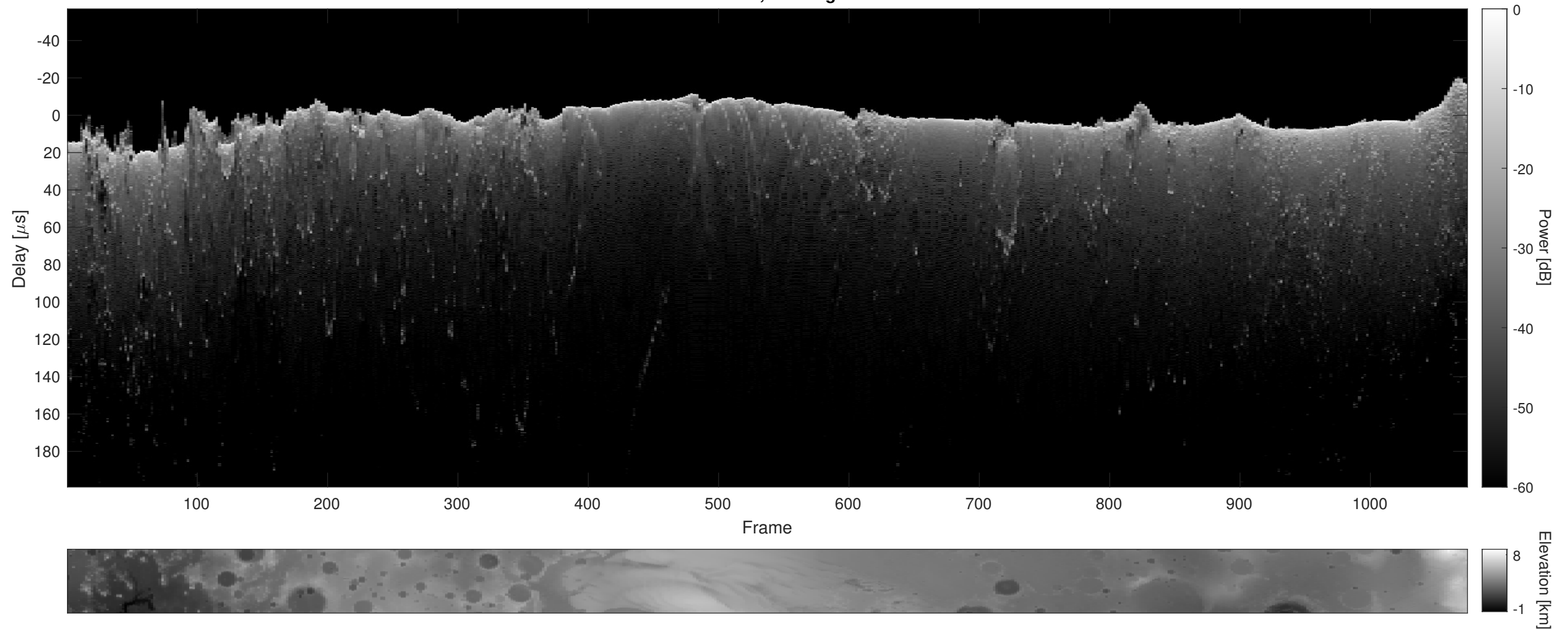
Orbit 10842, Cluttergram
