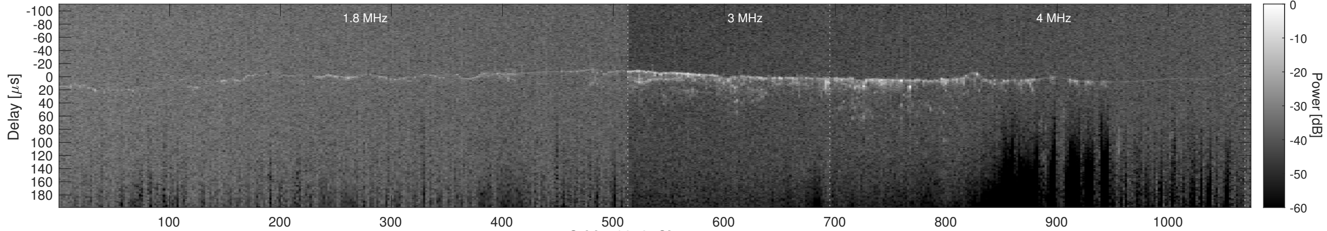
Orbit 10842, Cluttergram
