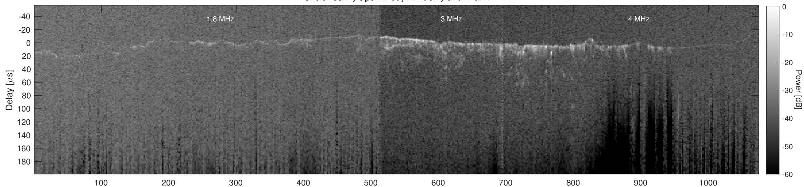
Orbit 10842, Cluttergram
