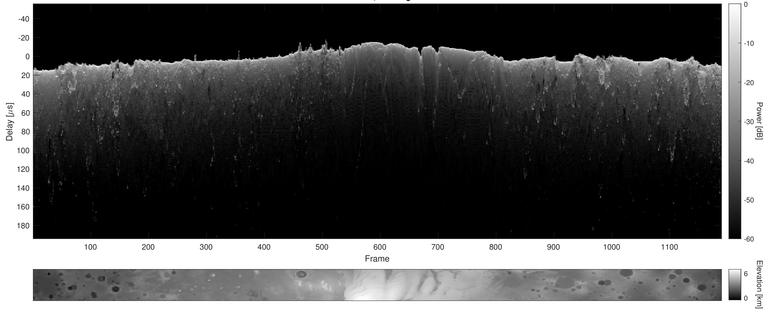
Orbit 10843, Cluttergram
