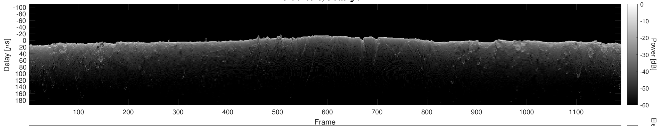
Orbit 10843, Cluttergram
