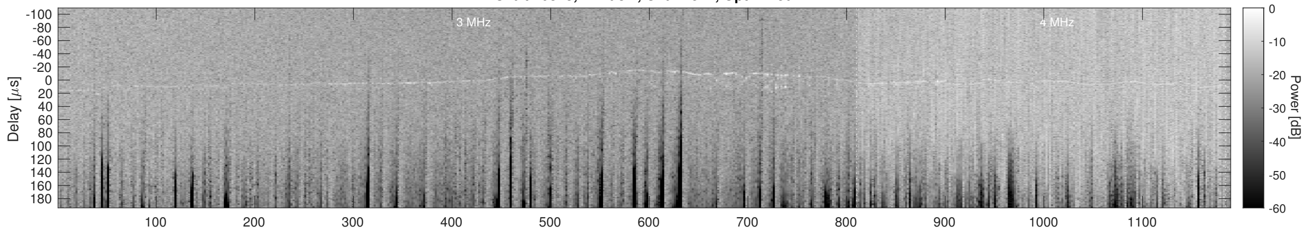
Orbit 10843, Cluttergram
