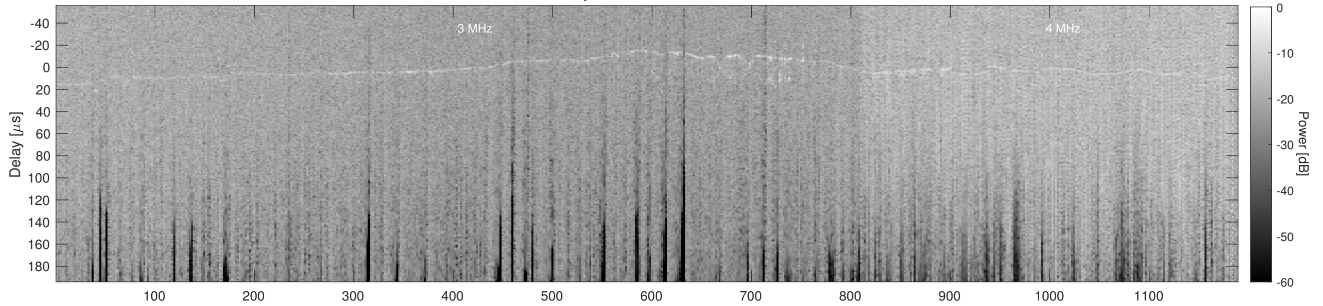
Orbit 10843, Cluttergram
