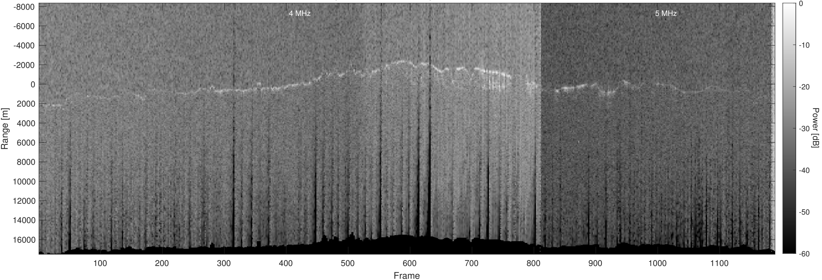
Orbit 10843, Optimized, Window, Depth-Corrected, Channel 2
