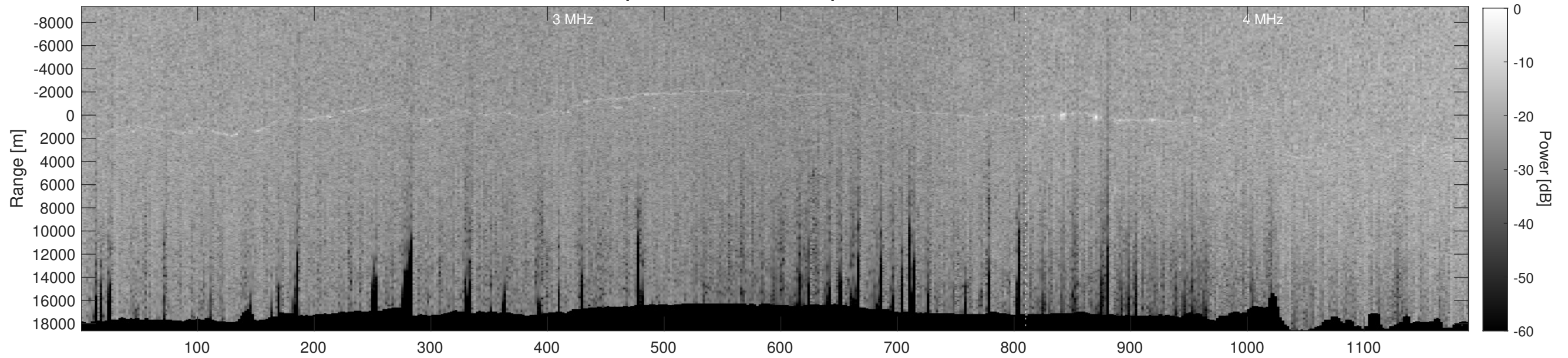
Orbit 10845, Depth-Corrected Cluttergram
