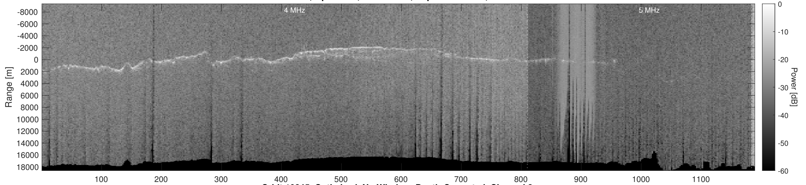
Orbit 10845, Optimized, No Window, Depth-Corrected, Channel 2
