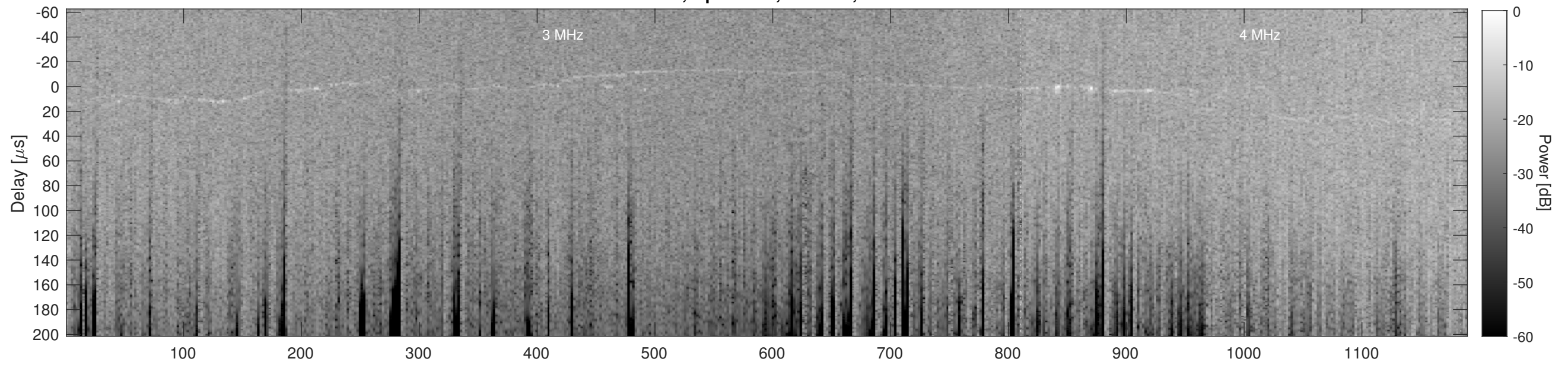
Orbit 10845, Cluttergram
