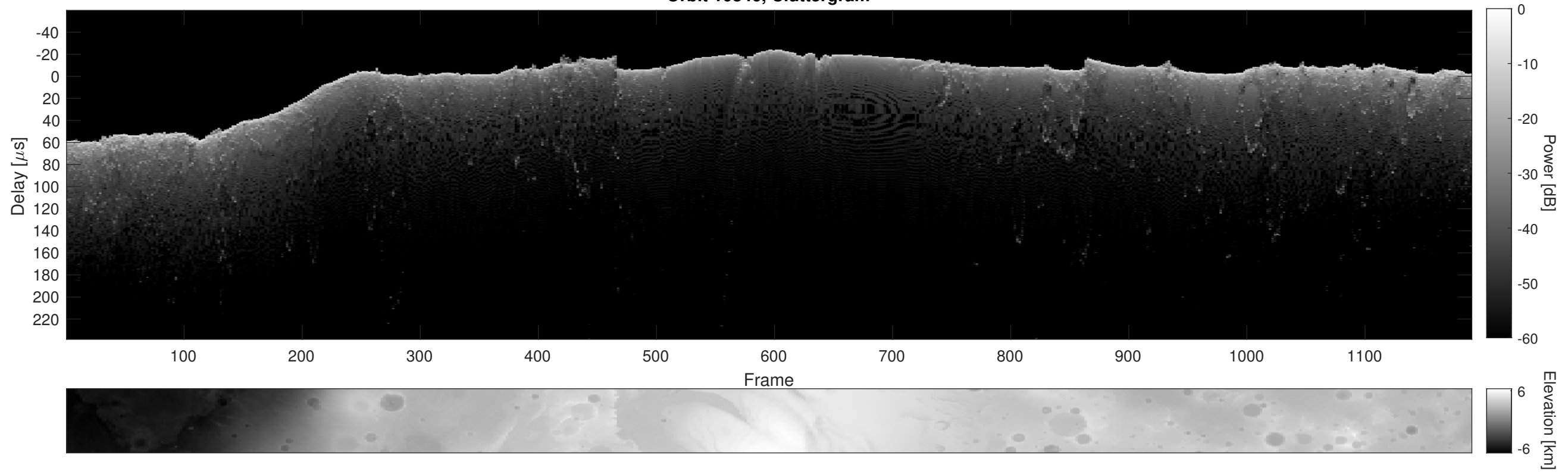
Orbit 10846, Cluttergram
