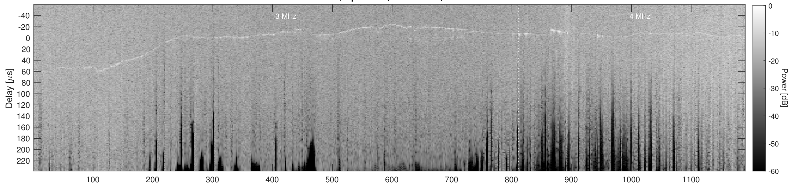
Orbit 10846, Cluttergram
