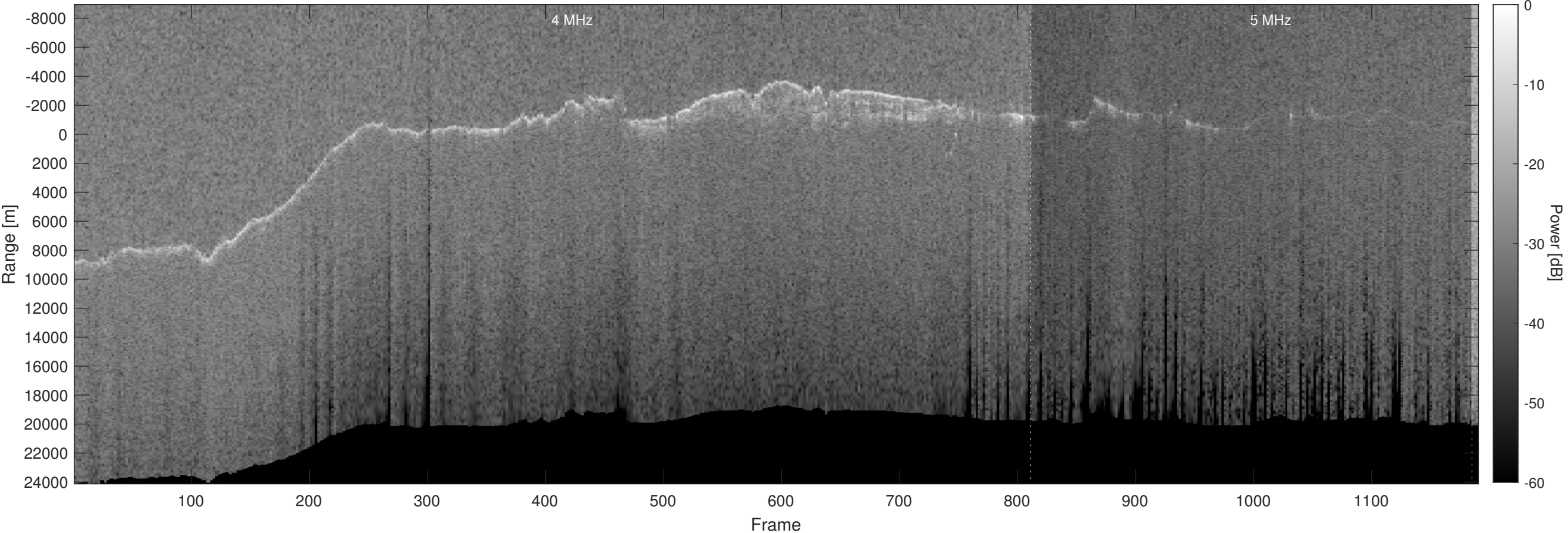
Orbit 10846, Optimized, No Window, Depth-Corrected, Channel 2
