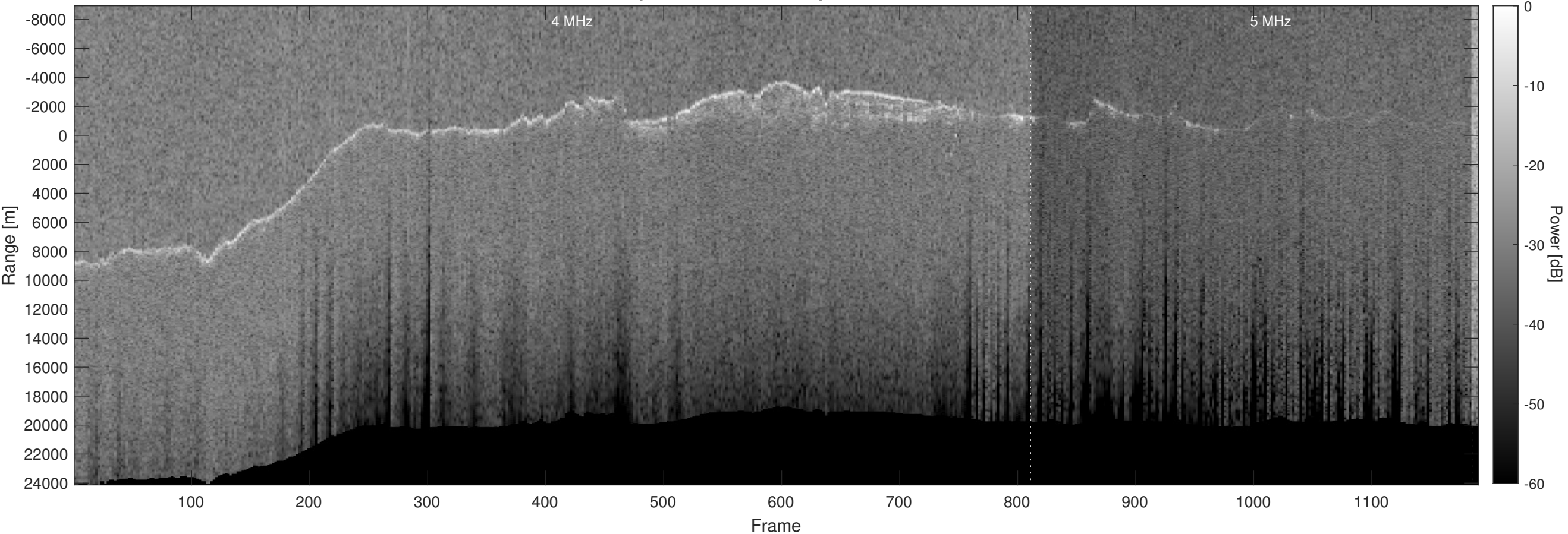
Orbit 10846, Optimized, Window, Depth-Corrected, Channel 2
