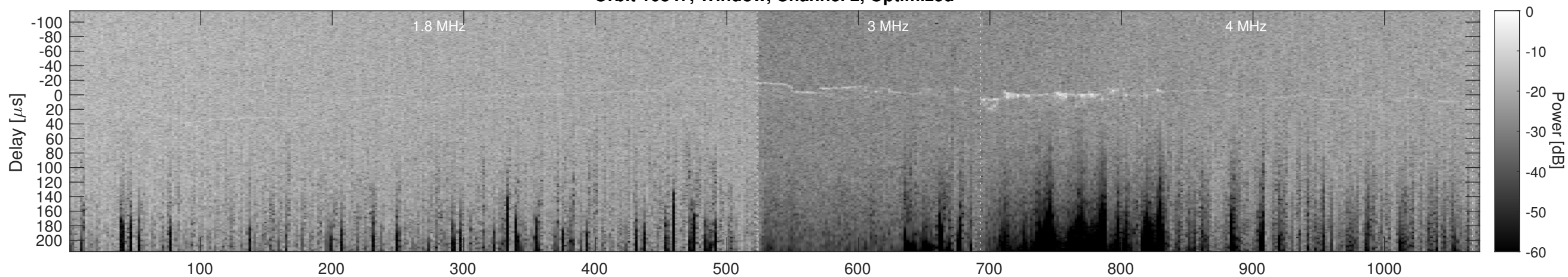
Orbit 10847, Cluttergram
