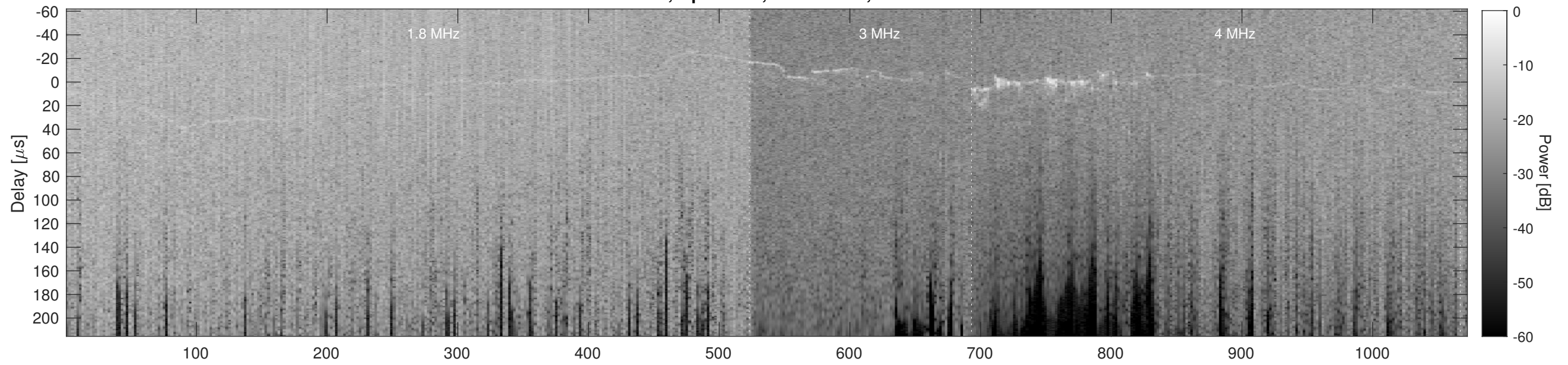
Orbit 10847, Cluttergram
