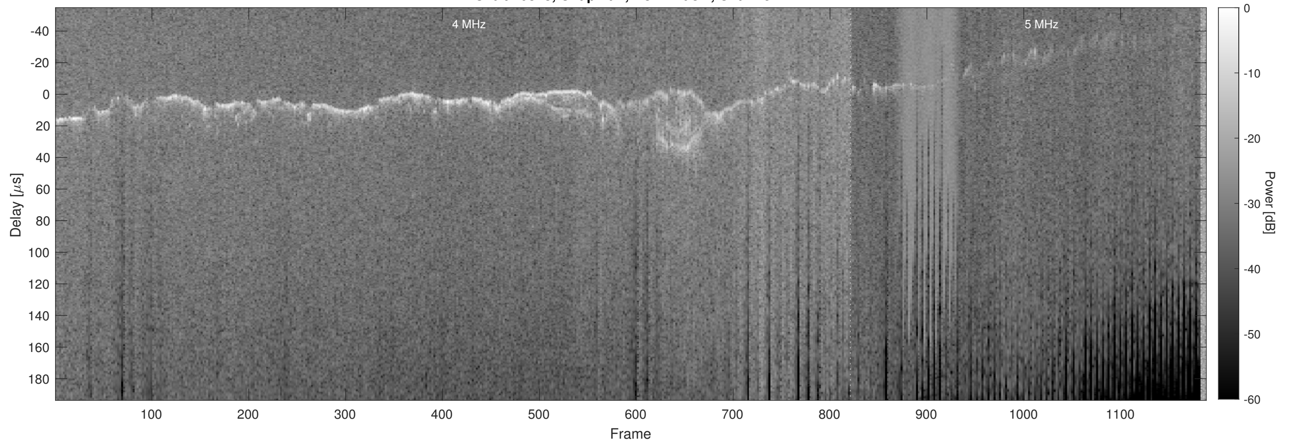
Orbit 10848, Chapman, No Window, Channel 2
