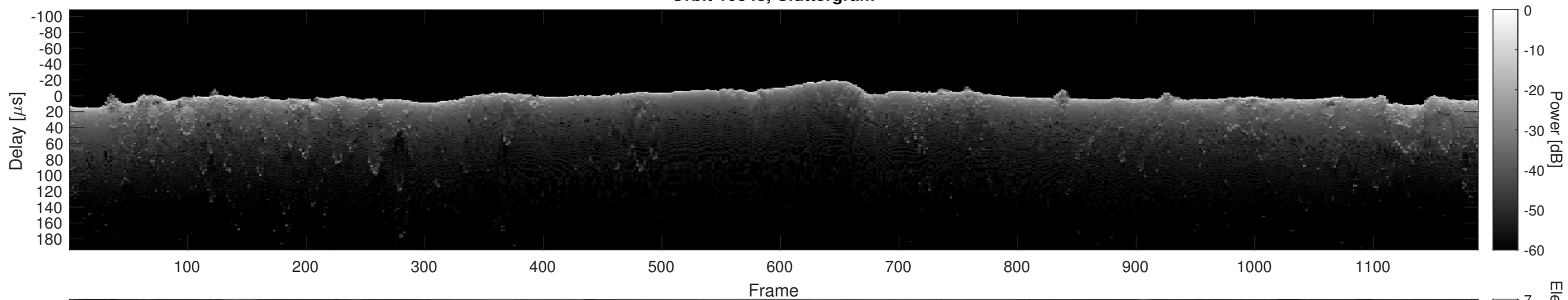
Orbit 10848, Cluttergram
