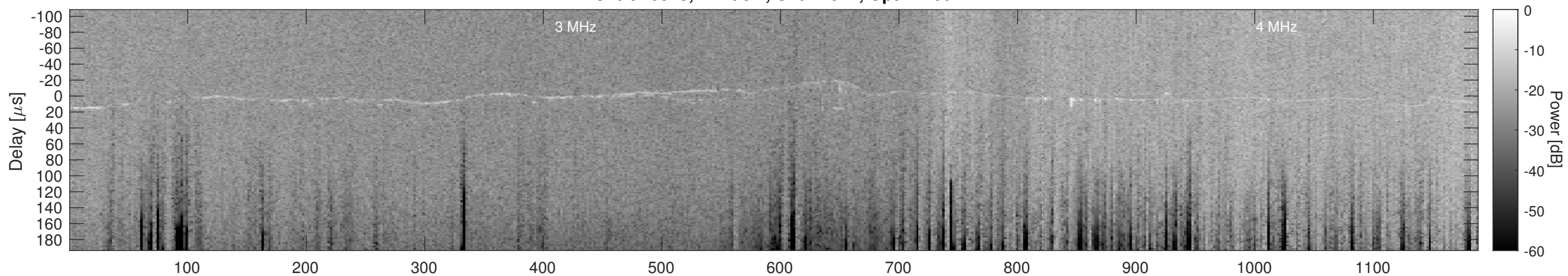
Orbit 10848, Cluttergram
