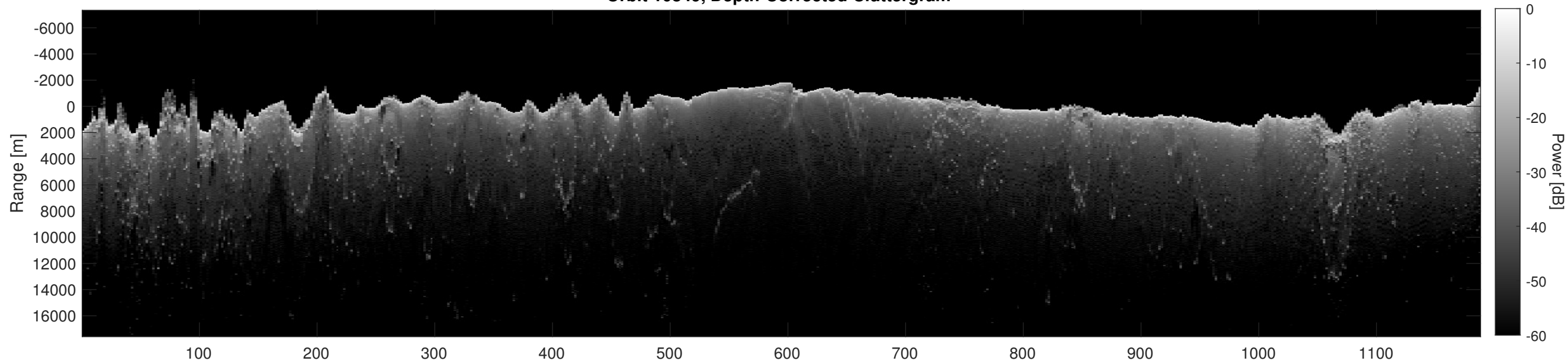
Orbit 10849, Depth-Corrected Cluttergram
