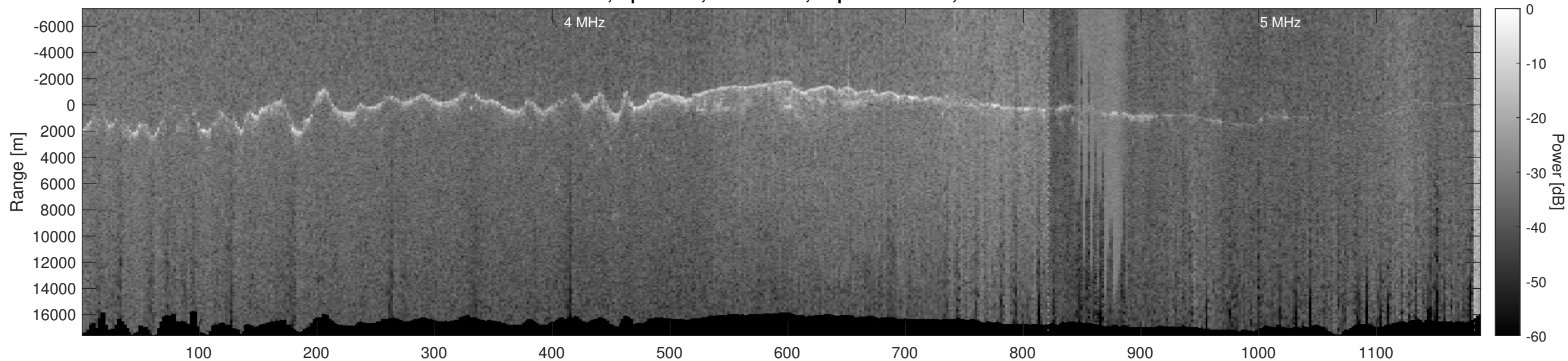
Orbit 10849, Optimized, No Window, Depth-Corrected, Channel 2
