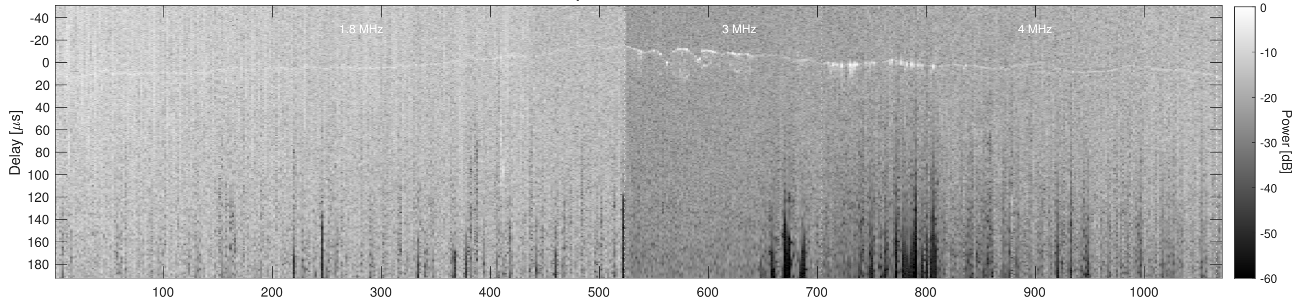
Orbit 10850, Cluttergram
