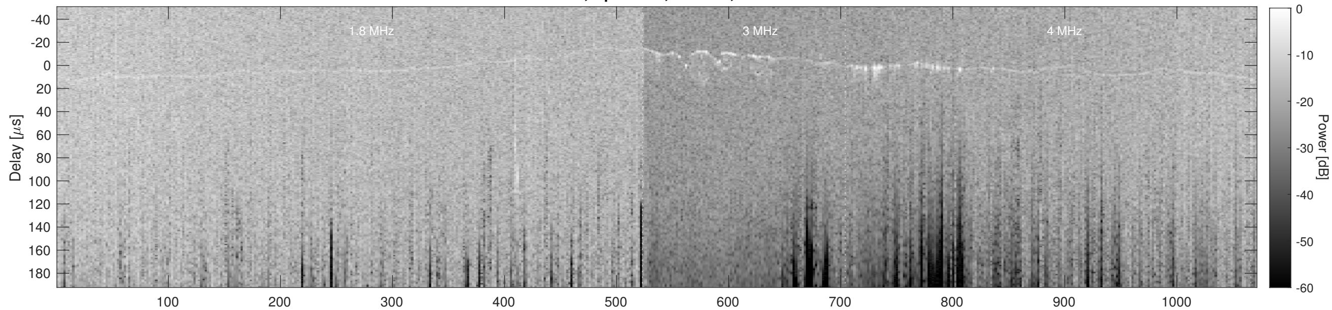
Orbit 10850, Cluttergram
