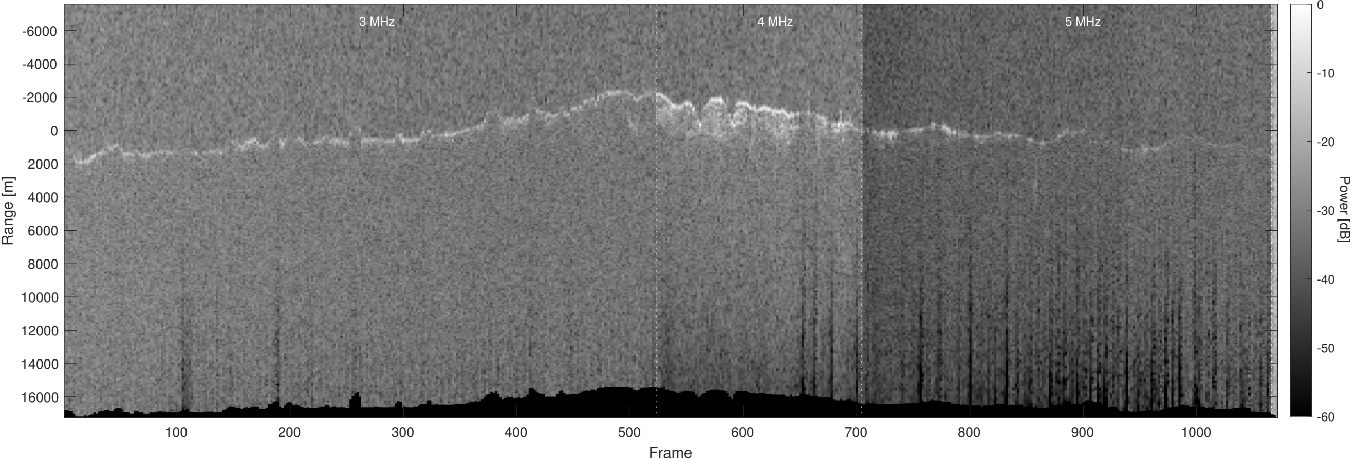
Orbit 10850, Optimized, Window, Depth-Corrected, Channel 2
