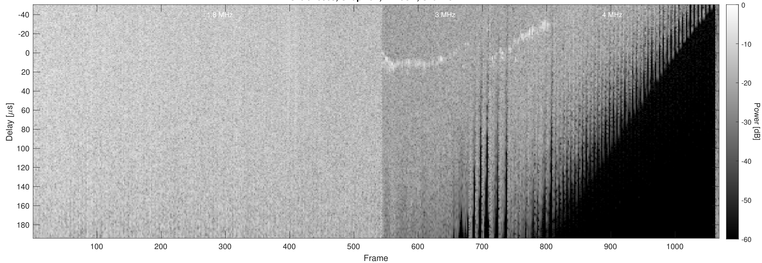
Orbit 10863, Chapman, Window, Channel 2
