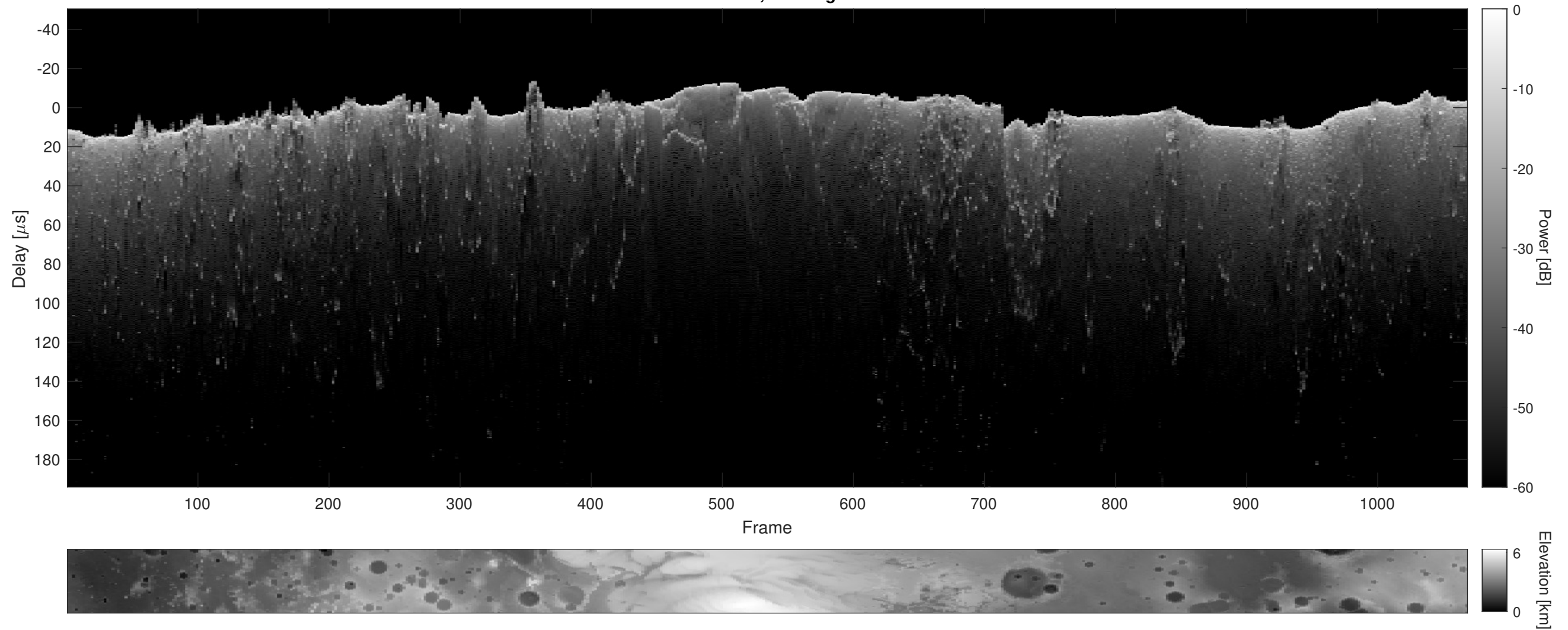
Orbit 10863, Cluttergram
