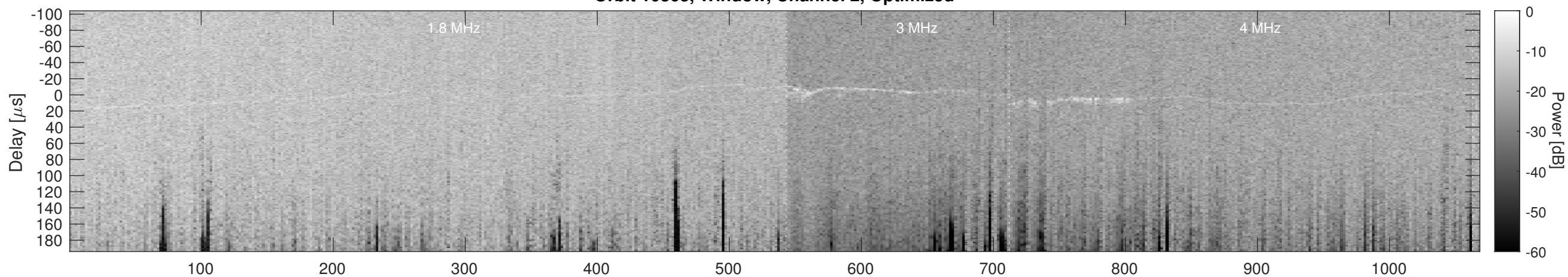
Orbit 10863, Cluttergram
