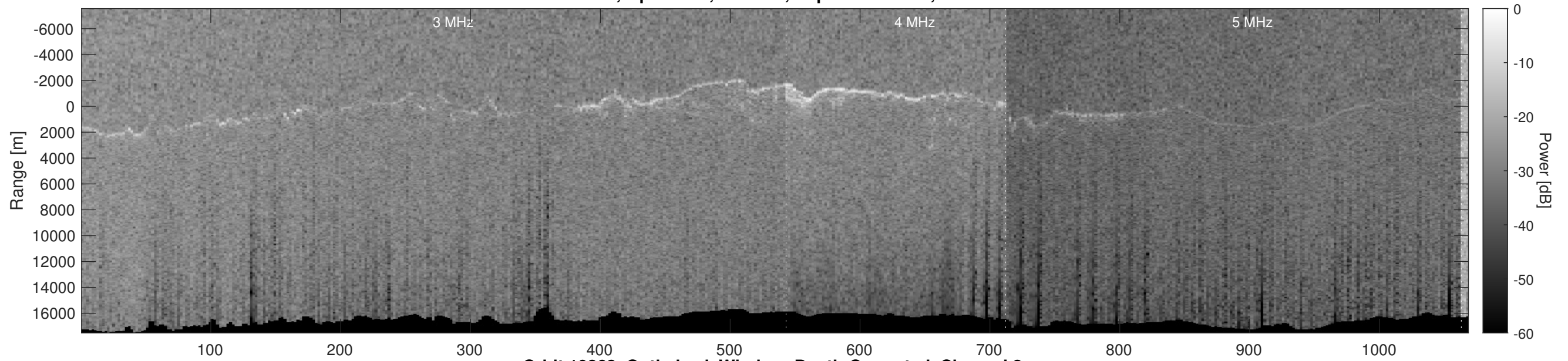
Orbit 10863, Optimized, Window, Depth-Corrected, Channel 2
