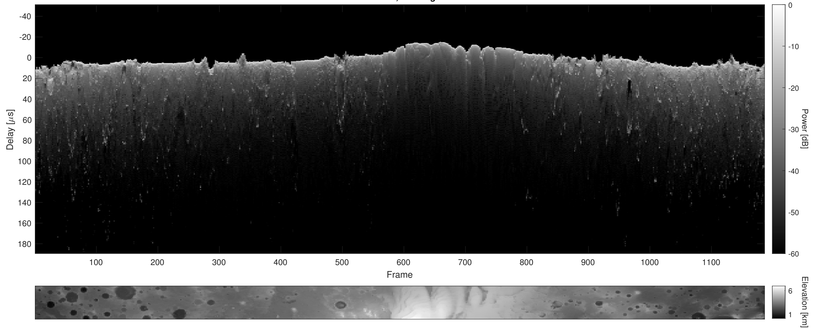
Orbit 10864, Cluttergram
