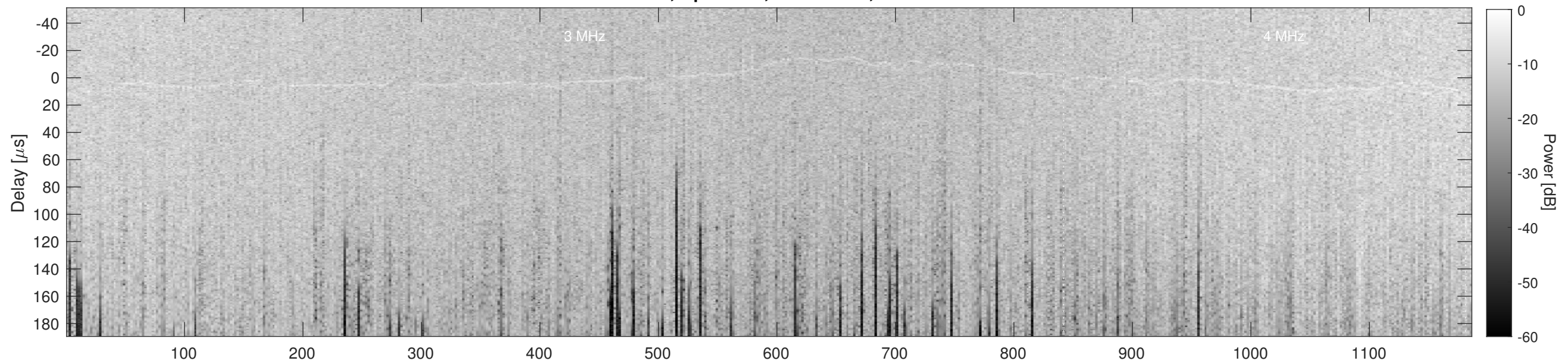
Orbit 10864, Cluttergram
